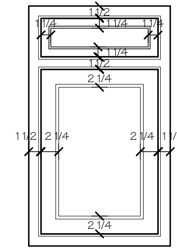
DOOR DETAIL SCALE: 1" = 1'
