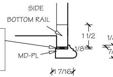
LIGHT VALANCE DETAIL SCALE: 3" = 1'
