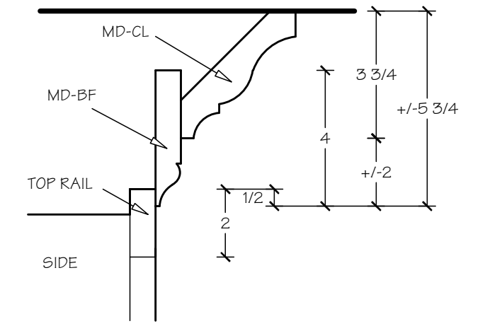
CROWN MOULDING DETAIL SCALE: 3" = 1'
